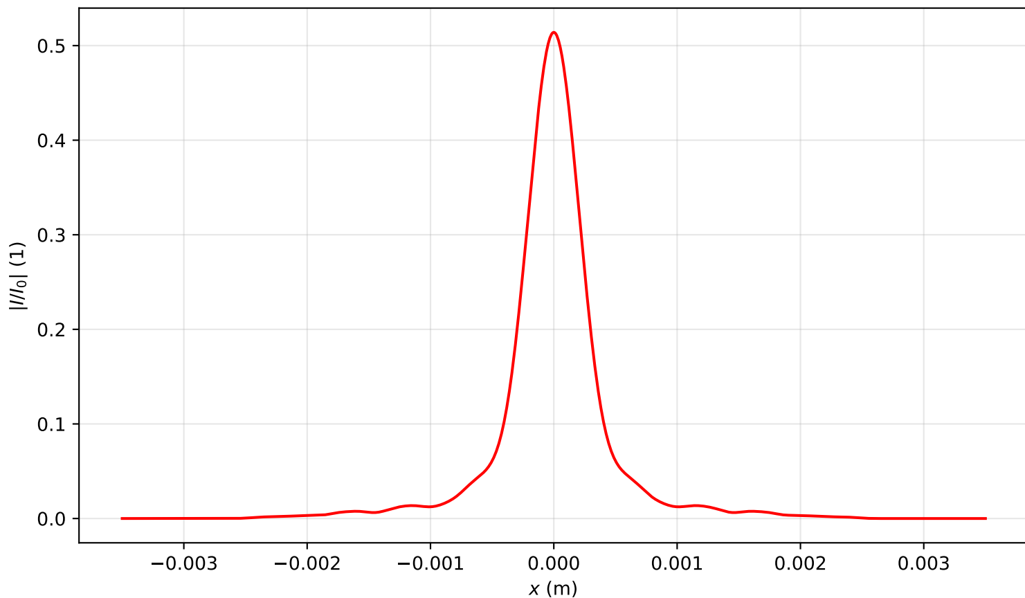
Intensity profile I(x, y = 0, z = 2.866)/I_0 , \text{Pin}=3.0\text{Pcr} , artificial time
